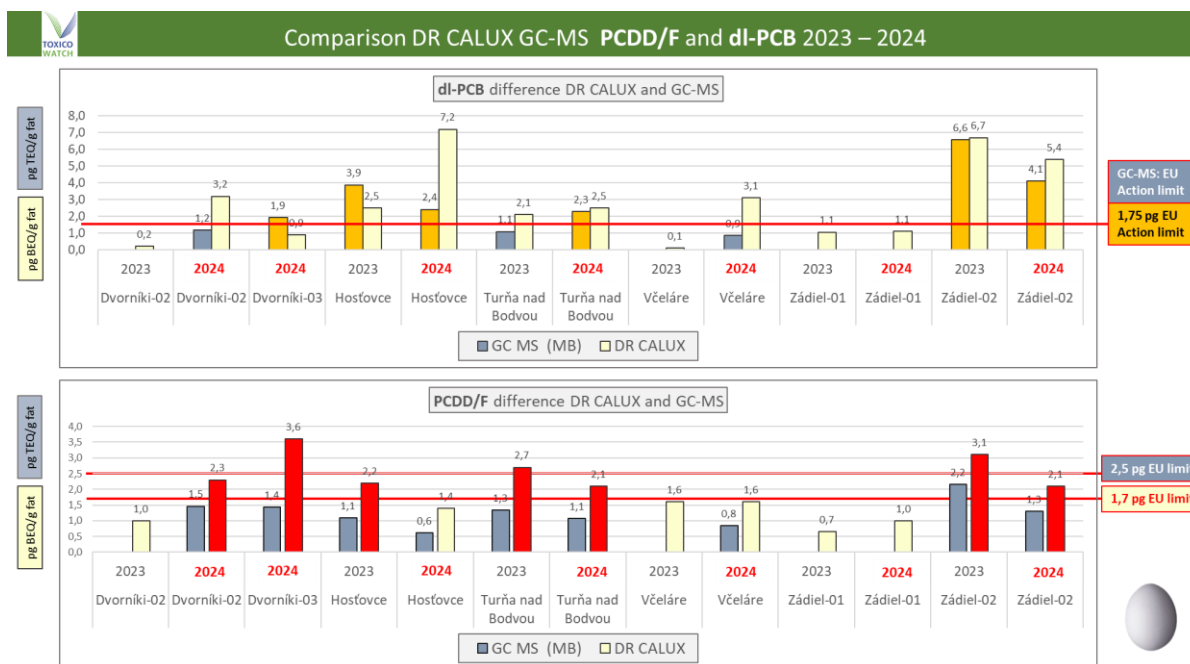
Figure 73: Comparison of chemical analyses and bioassay analyses on PCDD/F and dl-~PCB separately
