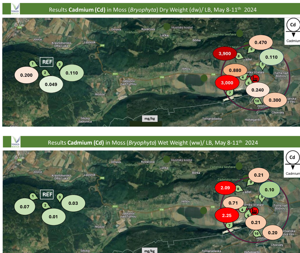
Figure 54: Results Cadmium (Cd) in moss expressed in dry (dm) and wet weight (ww) in mg/kg
