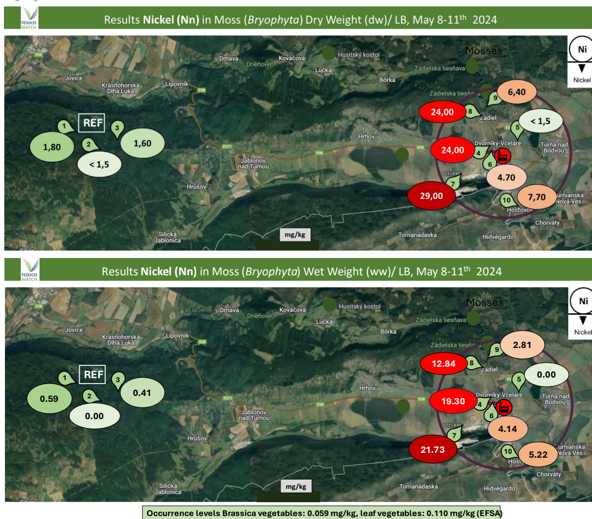
Figure 60: Results Nickel (Ni) in moss expressed in dry (dw) and wet weight (ww) in mg/kg
