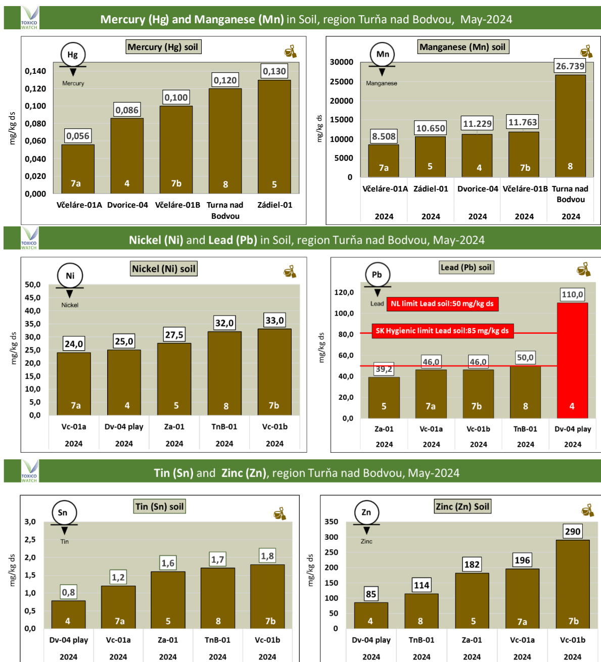
Figure 27: Results heavy metals Hg, Mn, Ni, Pb, Sn, Zn in soil, May 8-11th, 2024
