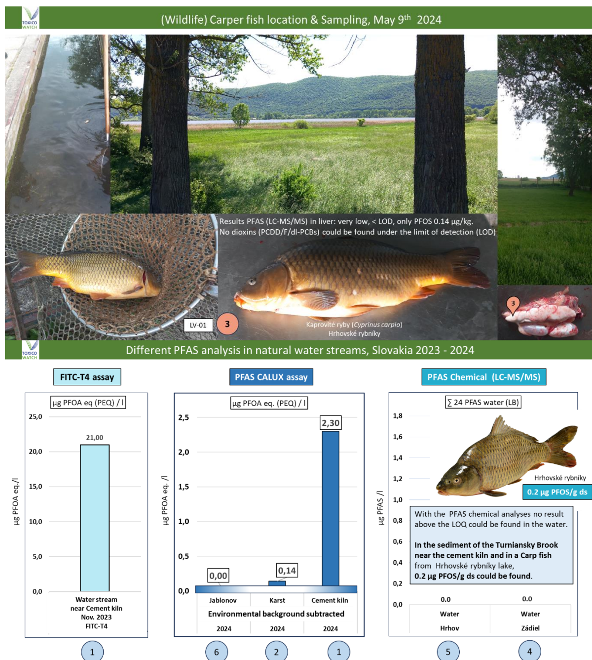
Figure 81: PFAS analyses in natural water streams
