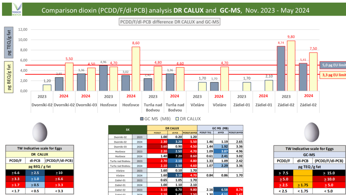
Figure 72: Comparison of chemical analyses and bioassay analyses on PCDD/F/dl-~PCB
