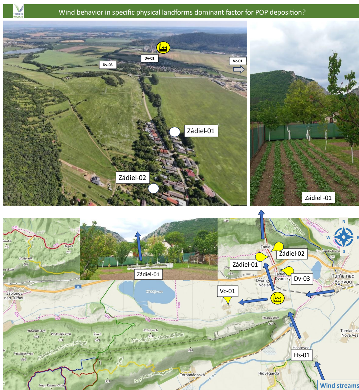
Figure 64: Wind behavior in specific physical landforms Zádíel
