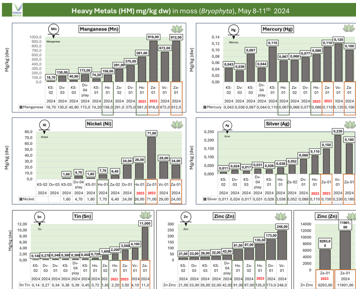
Figure 48: Results of heavy metals-14 in mosses ( Bryophyta ), May 8-11 th 2024
