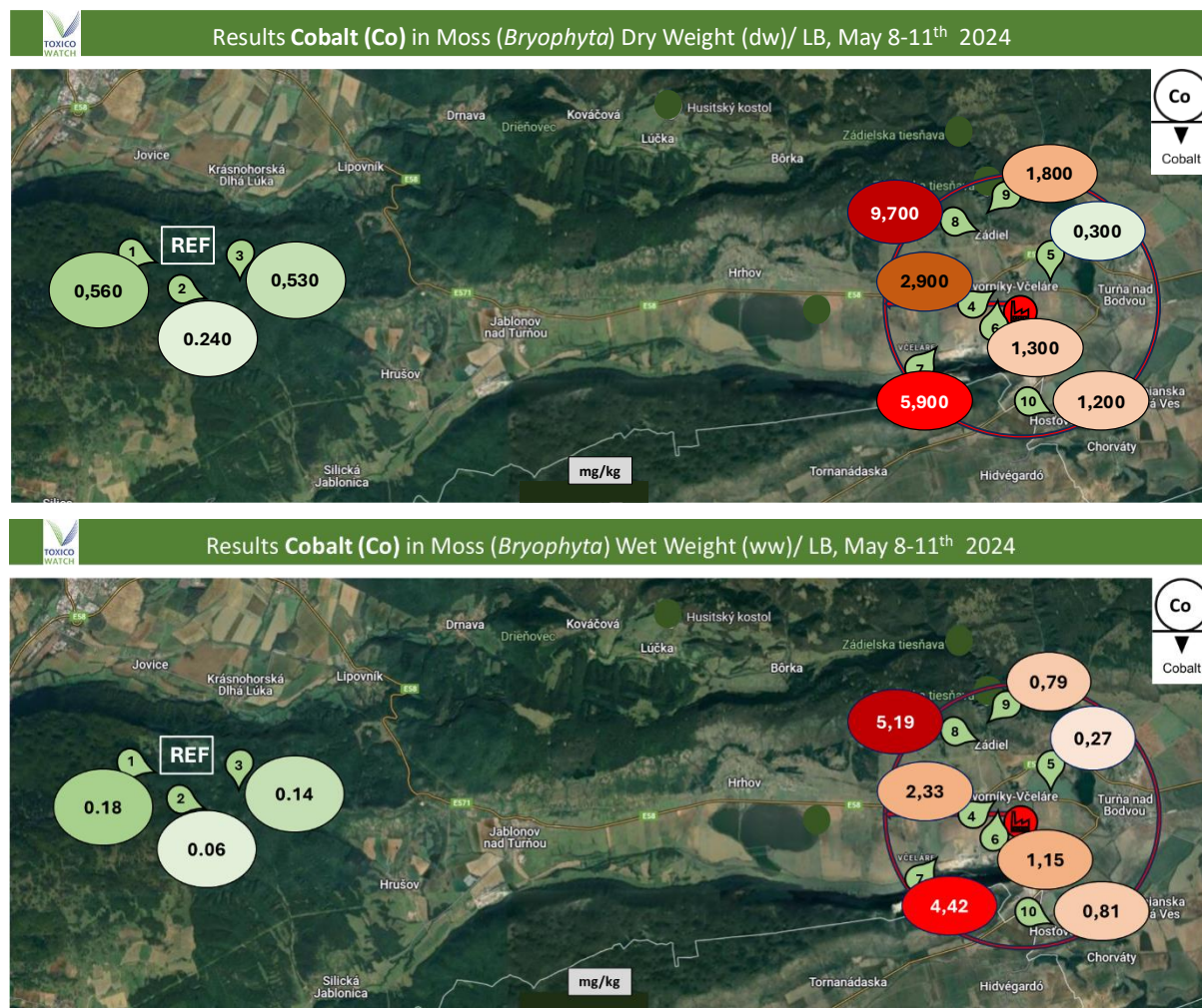
Figure 55: Results Cobalt (Co) in moss expressed in dry (dm) and wet weight (ww) in mg/kg
