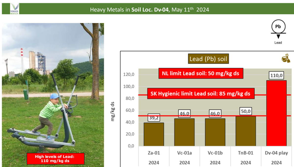
Figure 22: Heavy metal, Lead (Pb) in soil, location Dv-04, 2024
