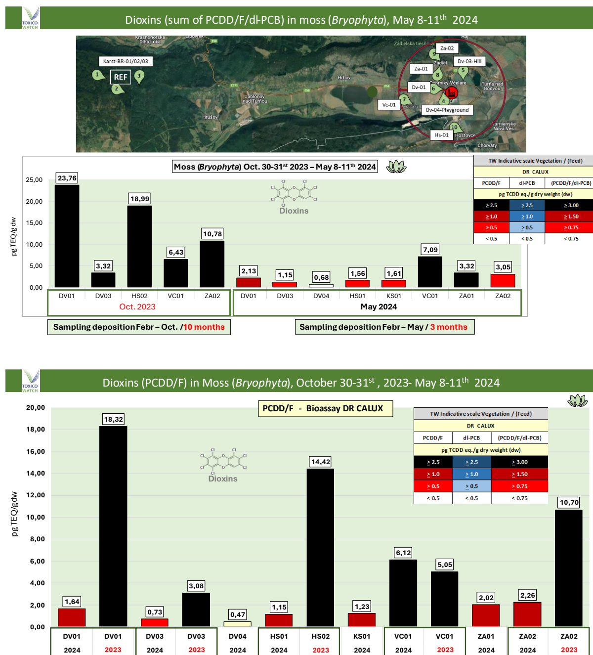
Figure 45: Results (sum) of dioxins (PCDD/F/dl-PCB) in mosses ( Bryophyta ), May 8-11 th 2024
